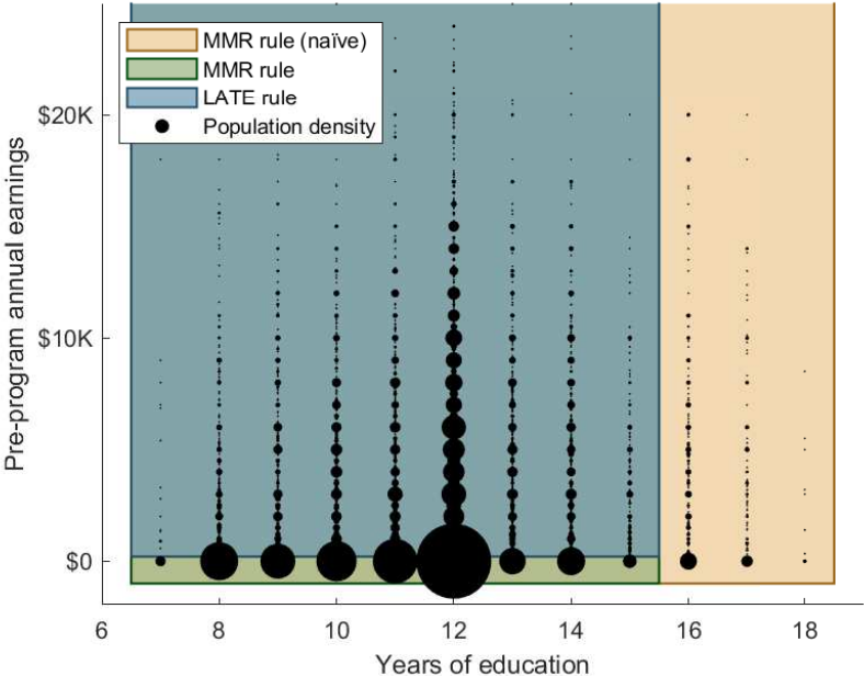
Figure 3: Estimated optimal policies from the quadrant policy class conditioning on years of education and pre-programme earnings.
