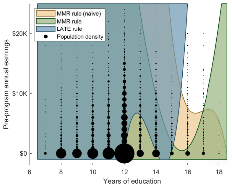
Figure 5: Estimated optimal policies from the linear-index policy class conditioning on years of education, (\text{education})^2 , (\text{education})^3 , and pre-programme earnings.
